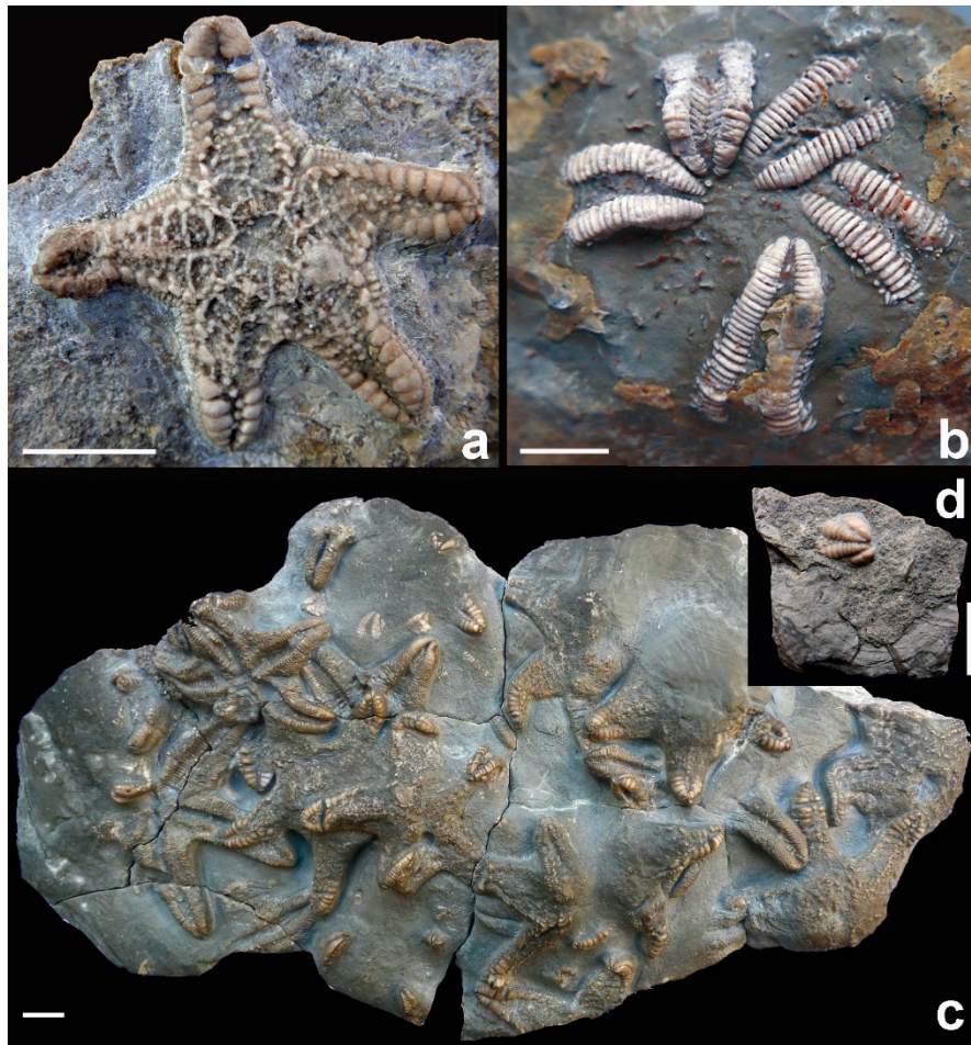
Fig. 2: Asteroid ( Trichasteropsis weissmanni ) conservation lagerstätten. a dorsoventrally compressed, on top of thick skeletal shell bed. Meißner Formation (nodosus biozone), Bölgental (Baden-Württemberg, Germany). MHI 843/1. b in concretion (Bindlach Type), dorsally arms recurved, outside nodule (nodosus biozone), Bayreuth-Bindlach (Upper Franconia, Bavaria, Germany). MHI 1857/22. c individuals transported and deposited both ventral and dorsal sides up, arms of some individuals recurved. nodosus biozone, Rothenburg-Gattenhofen (Middle Franconia, Bavaria, Germany). MHI 2062/1. d autotomized arm tip. Trochitenkalk Formation (pulcher biozone), Crailsheim-Wollmershausen (Baden-Württemberg, Germany). MHI 770/2. Scale bars 10 mm.
